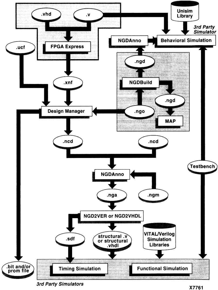
Figure B-1 Alliance FPGA Express/Xilinx Design Flow
