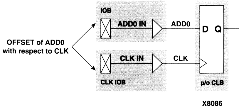
Figure H-3 Using OFFSET Constraints
