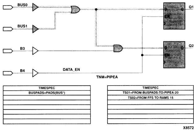
Figure H-4 Example TNM, TIMESPEC, and TIMEGRP
