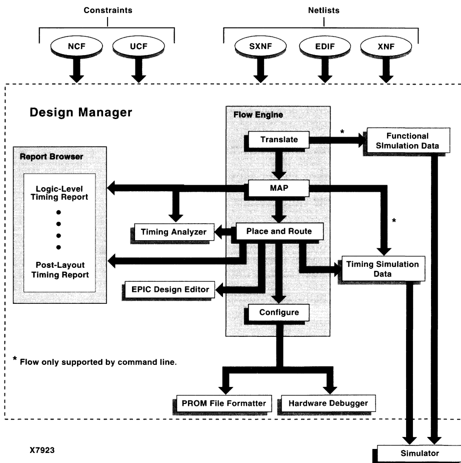
Figure 4-1 Xilinx Design Flow
