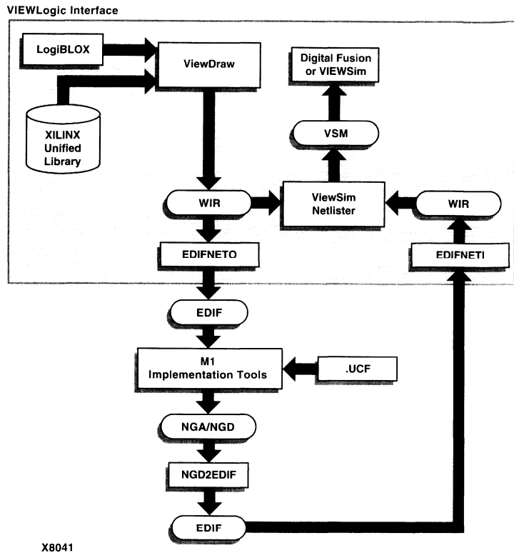
Figure E-1 Viewlogic/Xilinx Software Design Flow
