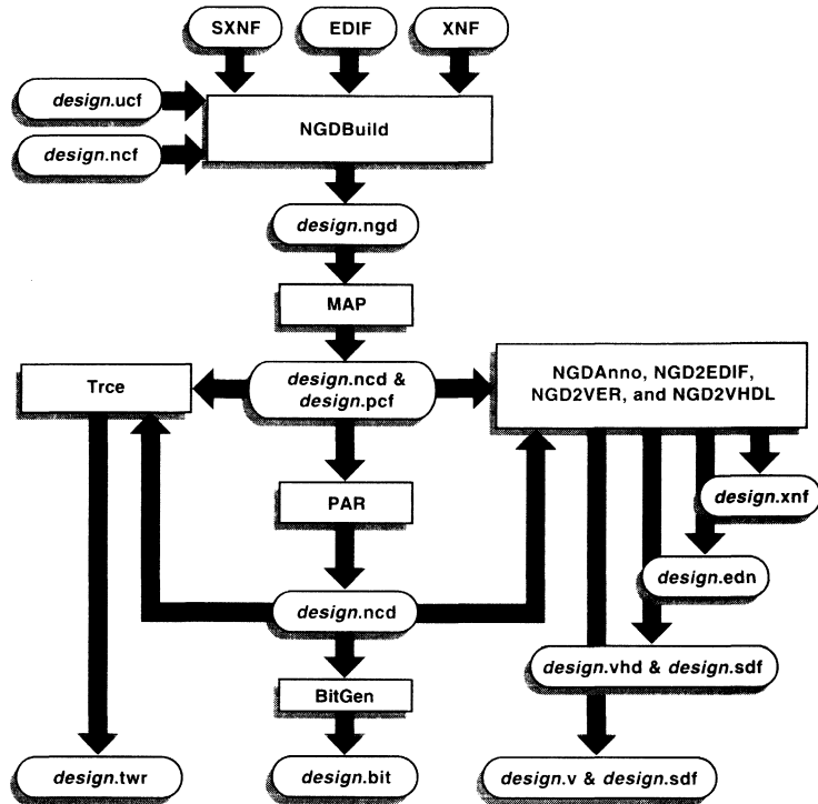
Figure 4-2 Detailed Design Flow
