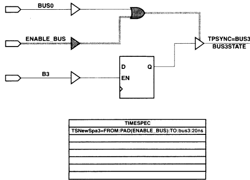
Figure H-5 TPSYNC Example
