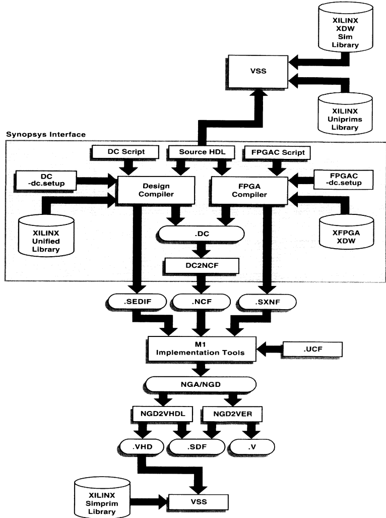
Figure D-1 XSI Design Flow
