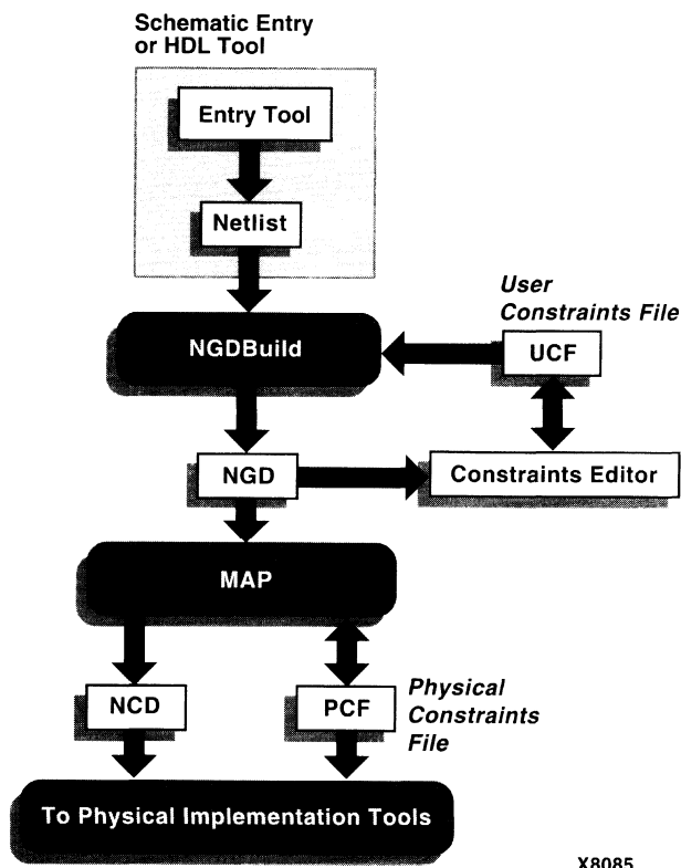
Figure H-1 Entering Design Constraints
