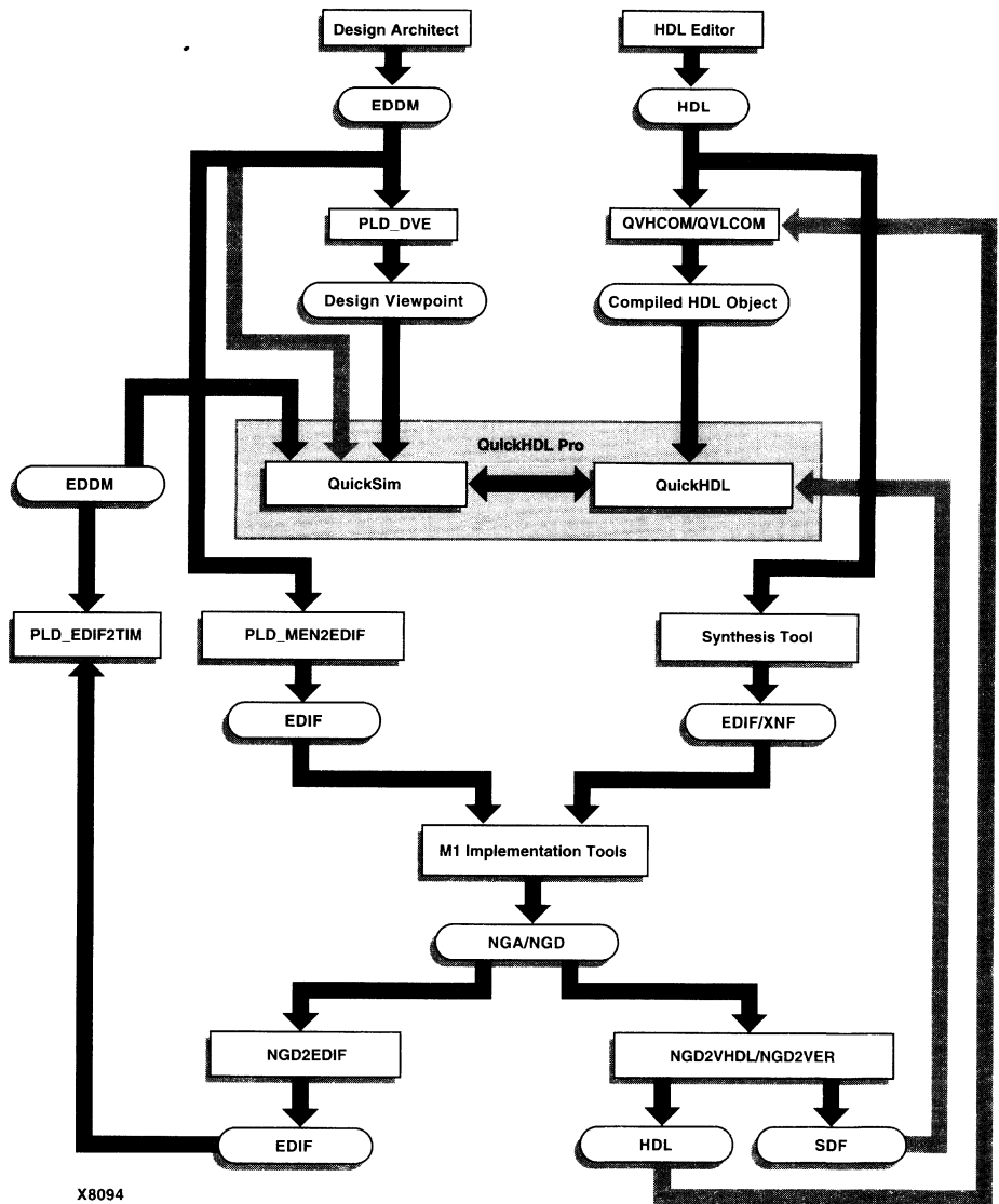
Figure C-1 Mentor/Xilinx Software Flow
